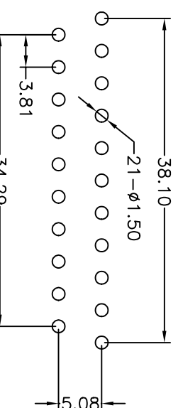
RECOMMEND P.C. BOARD LAYOUT
